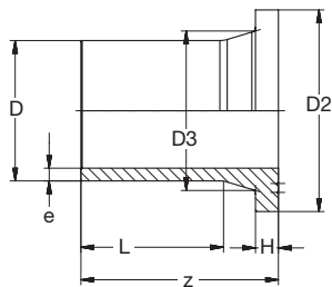
25.80.01.103 PE100 V-Bund lang gerillt SDR11 schwarz PE100 Flange adaptor spigot long grooved SDR11 black
